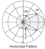
Horizontal Pattern
