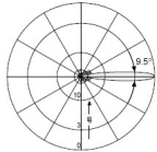
Vertical Pattern
